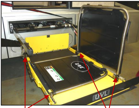
Pins must be set at ends of each side panel
